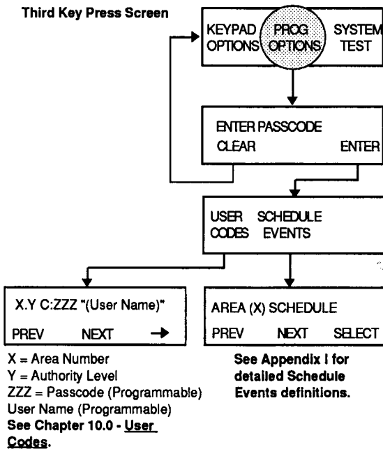
FIGURE 23 - PROGRAMMING OPTIONS PROCEDURE
